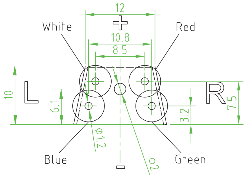
Blue: LH Earth / Green: RH Earth / Red: RH Signal / White: LH Signal
